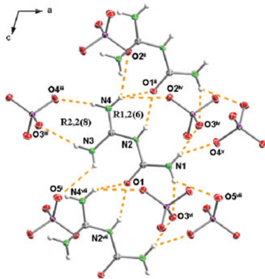
FIGURE 3 View along the b axis of the hydrogen bonding around the guanyluurea cation in GUP (symmetry codes: (i) x, -y + 1/2, z + 1/2 ; (ii) x, -y + 1/2, z - 1/2 ; (iii) -x - 1, y - 1/2, -z + 1/2 ; (iv) -x, y - 1/2, -z + 1/2 ; (v) +1, y, z ; (vi) -x, -y + 1, -z + 1 ; (vii) x + 1, -y + 1/2, z + 1/2 ).
